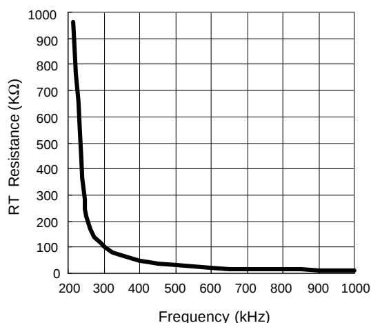
Figure3. Oscillator Frequency vs. RT Resistance (High Frequency)
