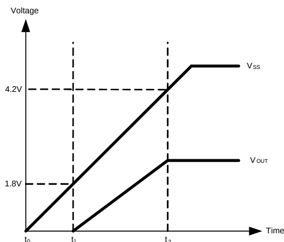
Figure 1. Soft-Start Interval
