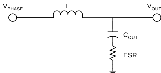
Figure 5. The Output LC Filter
